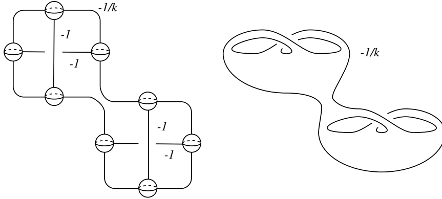
FIGURE 2. Two handle diagrams of the manifold M' .
