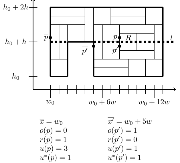
Figure 6: An h -region P and a rectangle R crossing a slicing line illustrating the definitions r(p) , o(p) , u(p) , and u^*(p) .
