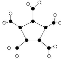
Figure 7. A pentagon with 10 vertices with 10 external legs.
