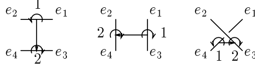
Figure 3. Three graphs I, H, X together with their total ordering, where shown are particular orderings of the trivalent vertices together with flag orientations for the respective vertices and internal edges. The external edges e_1, \dots, e_4 are assumed (flag-)oriented in the same way on the three graphs.
