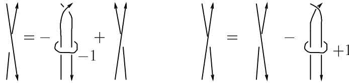
Figure 5. Another special case of equation (13). The figure represents an identity in \mathcal{M} . There are two interpretations of the above figure. Either each of the crossings shown belong to the same component (of an algebraically split link), or each of the crossings shown are part of a ribbon of a piece of a Seifert surface of a 1-pair blink. It will be clear each time we use the identity shown in the figure which interpretation we have in mind.
