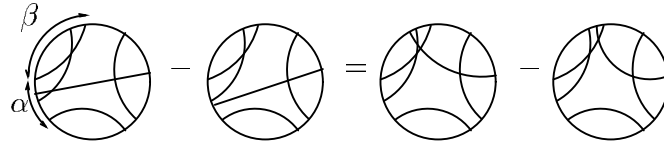
Figure 27. The 4-term relation with a fixed “special” chord and a moving “nonspecial” chord. For the convenience, the arcs \alpha, \beta are shown, too. The first two terms show a “nonspecial” chord after and before passing a special chord (in the \alpha arc). The two last terms have no “nonspecial” chord.
