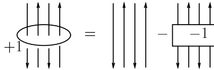
Figure 34. An equality in \mathcal{M} . The -1 in the box indicates a full twist. Notice that all arcs lie in the same link component, and that the two links shown on the right hand side of the figure are homotopic, and therefore, by doing a number of crossing changes we can rewrite the right hand side as a finite sum of terms each of which contains at least one disc that intersects the link component in two points.
