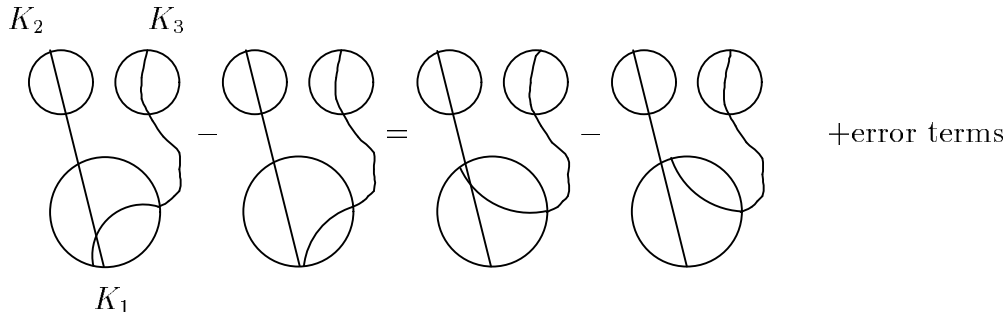
Figure 23. The third version of the 4-term relation on \mathcal{M} , with the notation of remark 3.11.
