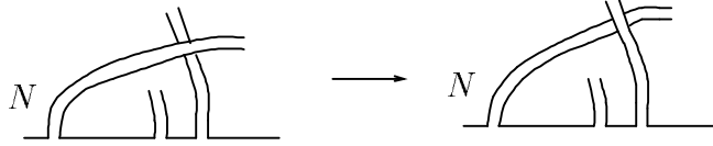
Figure 43. An illustration of an original homotopy.
