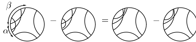
Figure 28. The 4-term relation with a fixed “special” chord and a moving “special” chord. For the convenience, the arcs \alpha, \beta are shown, too. The first two terms show a “special” chord after and before passing a fixed “special” chord (in the \alpha arc). The two last terms have chords that begin and end in the \beta arc, and therefore, by the discussion of step 3, we can find a 4-tower.
