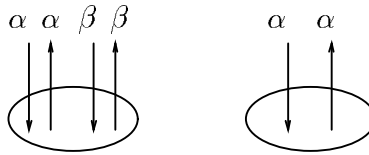
Figure 29. Shown here are the two allowable types of intersections of a disc D_i with the components of L' . Here \alpha, \beta denote components of L' and we assume that \alpha \neq \beta .
