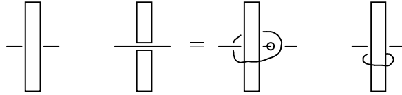
Figure 9. Another special case of equation (13). We assume that all the arcs in the band lie in the same link component. Then the link shown in the third picture from the left contains a unit Seifert-framed 1-pair blink (indeed, it bounds a Seifert surface obtained by tubing the obvious disc along the strands contained in the band). The fourth picture from the left contains a 1-component boundary link in the complement of the rest of the link, and thus (using remark 1.13) a 1-pair blink.
