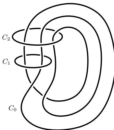
FIGURE 1.7. The link L .
