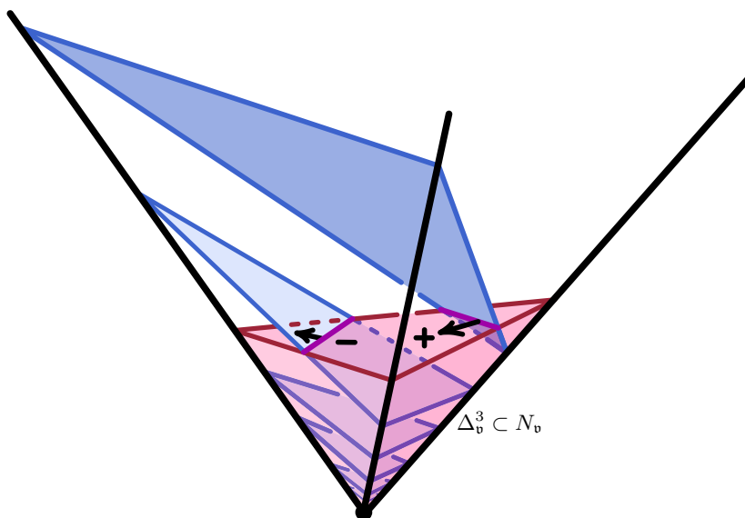
FIGURE 2.4. Orienting S \cap B_{\mathfrak{v}} . Notice that S meets the triangle of B_{\mathfrak{v}} in at most two of the three possible types of normal arcs.
