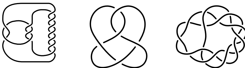
FIGURE 1.8. The (-2, 3, 7) pretzel, the 5_2 knot, and the k_4_3 knot.
