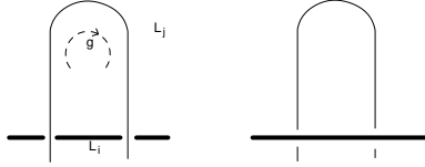
Figure 3. A double crossing change.
