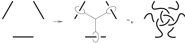
Figure 4. A \Delta -move.
