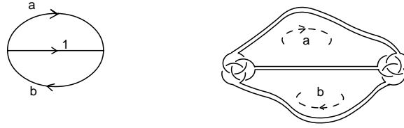
Figure 9. An edge and vertex oriented diagram and the associated \pi -AS link.
