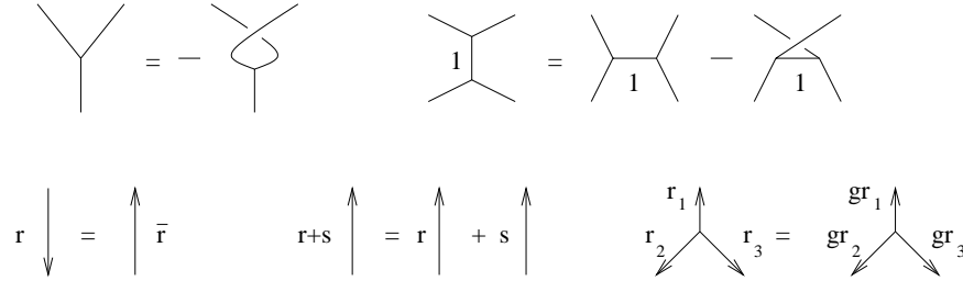
Figure 2. The AS, IHX, R_1 , R_2 and R_3 relations. Here \bar{g} = g^{-1} is the involution of \mathbb{Z}\pi , r, s, r_i \in \mathbb{Z}\pi and g \in \pi .
