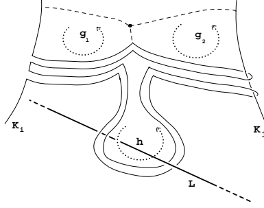
Figure 1. Modification of a link.
