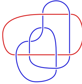
Fig. 2. The link 9^2_{34} .
