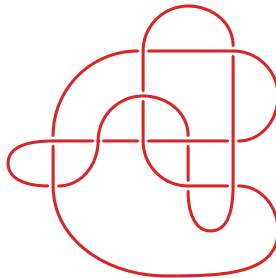
Fig. 1. The knot K11n116 .
