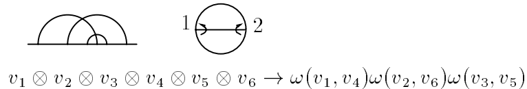
Figure 4. A degree 3 linear chord diagram and its associated trivalent graph. The trivalent graph G comes equipped with an ordering od_{V(G)} of its vertices, as well as with a vertex orientation or_{V(G)} , indicated by a choice of cyclic order of the edges around each vertex. The linear chord diagram corresponds (under the map (33)) to the contraction shown \otimes^6 H \rightarrow \mathbb{Q} shown in the figure.
