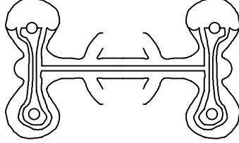
Figure 17. The connected sum of two b labeled curves is a bounding curve. Thus Dehn surgery along it represents an element of \mathcal{K}_g .
