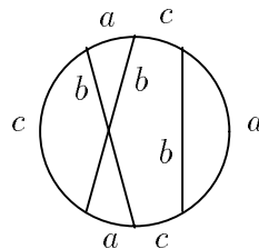
Figure 16. A labeling of the edges of a degree 3 chord diagram with labels a, b, c .
