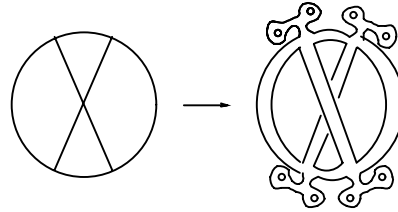
Figure 15. For the chord diagram , shown on the left, the construction of a handlebody \Sigma_\Gamma on the right.
