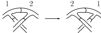
Figure 18. An isotopy of the handlebody on the left to the handlebody on the right via a handle slide.
