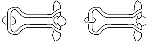
Figure 14. The links shown above associated to any nontrivial permutation of a, b, c are trivial.
