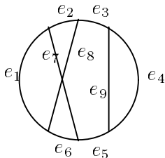
Figure 11. A degree 3 chord diagram on a circle.
