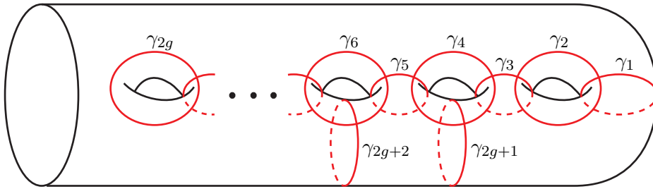
FIGURE 1. A surface \Sigma of genus g with one boundary component and 2g + 2 curves marked.
