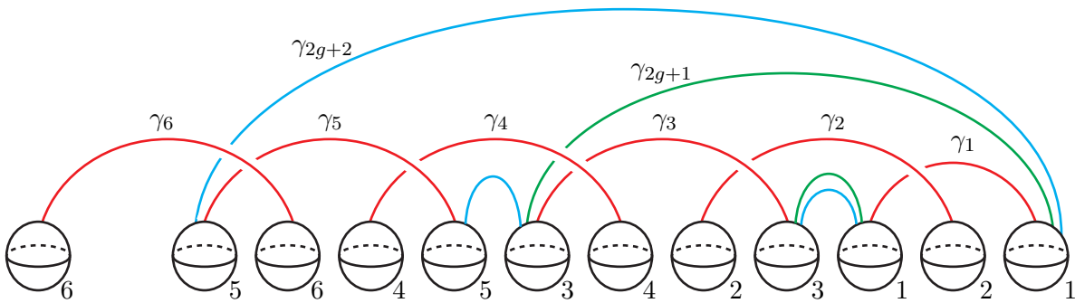
FIGURE 2. Handle presentation describing manifolds in Proposition 2.7 when the genus is 3. All 2-handles have framing -1 . The 1-handles are paired as indicated by the numbers.
