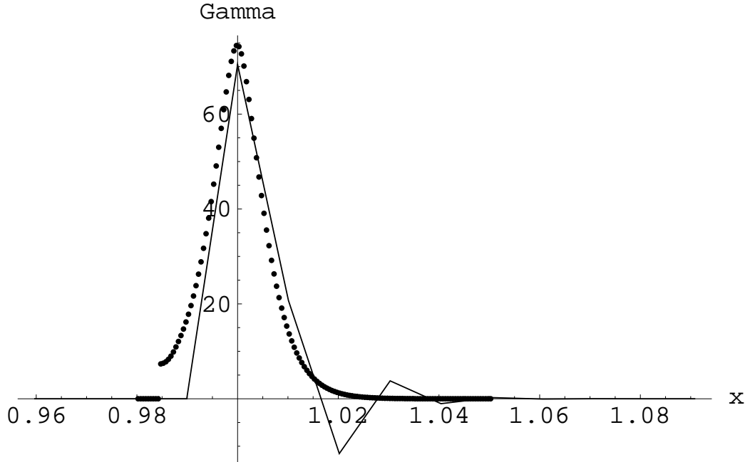
Fig. 1. Gamma for an American put near the free boundary.
