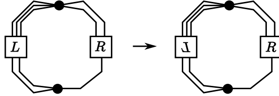
Figure 4. A Whitney flip on a graph.
