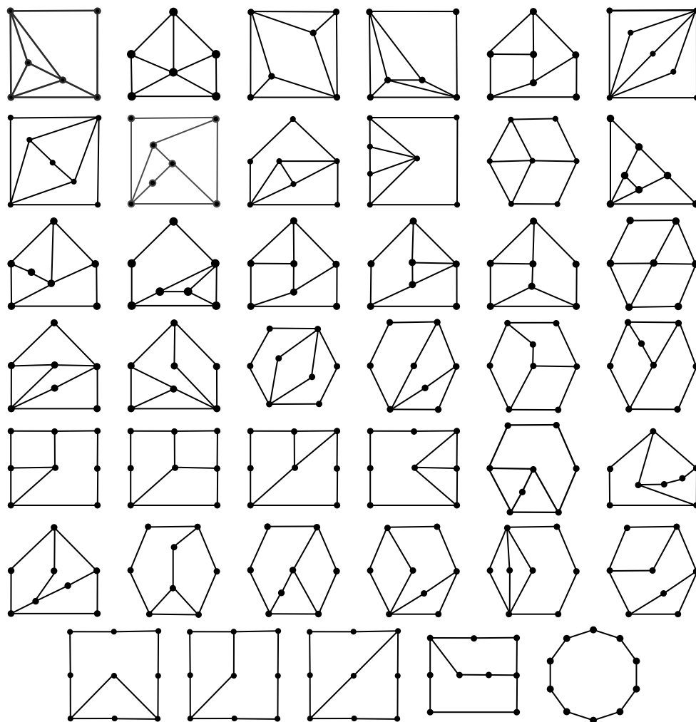
Figure 16. The irreducible planar graphs with 10 edges: G_0^{10}, \dots, G_5^{10} on the top, G_6^{10}, \dots, G_{35}^{10} on the middle and G_{36}^{10}, \dots, G_{40}^{10} on the bottom.
