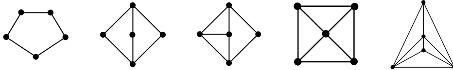
Figure 10. The irreducible planar graphs Gv_i^5 for i = 1, \dots, 5 (from the left to the right) with 5 vertices.
