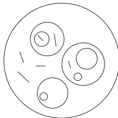
Figure 11. An intersection of a disc with the surface \Sigma_b
