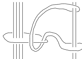
Figure 3. Shown here is the intersection of U with the link L_{twist} . Note that L_{twist} - L \subseteq U .
