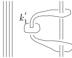
Figure 2. Shown here is the intersection of U with the link L_\alpha obtained by changing k_1 to k'_1 . Note that L_\alpha - L \subseteq U .
