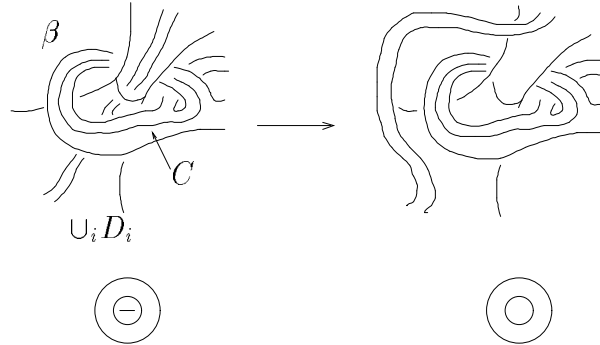
Figure 12. In the left side of this picture is shown a band \beta that does not penetrate any of the discs D_i , its associated circle C . The disc which the circle C bounds intersects the union \cup_i D_i as shown in the lower part of the left hand side. After a band change move, shown on the right hand side, we can arrange so that the new disc of the new circle has one less band intersection with the union of the discs \cup_i D_i .
