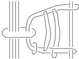
Figure 6. Yet another intersection of U with a link.
