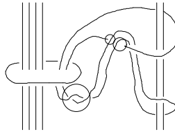
Figure 5. Shown here is an isotopy fixing the boundary of the intersection of U with the link L_{twist} . Note that L_{twist} - L \subseteq U . Also circled are 3 crossings to be changed.
