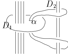
Figure 1. Shown here is the intersection of L with U . Note that k_i = \partial D_i for i = 1, 2 . and that the discs D_1 and D_2 intersect in an ribbon arc \alpha .
