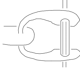
Figure 13. An intersection of L with U . Shown also is the genus 1 surface \Sigma_j .
