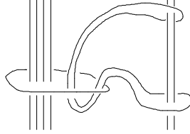
Figure 4. Shown here is the intersection of U with the link L_{untwist} . Note that L_{untwist} - L \subseteq U .
