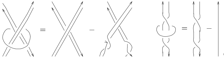
Figure 9. A few more identities in \mathcal{M}
