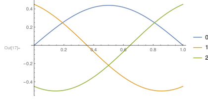
FIGURE 2. A plot of the growth rates \operatorname{Re}(\operatorname{Vol}_{\mathbb{C}}(\rho_j)/2\pi i\tau) of w^{(\sigma_j)}(x) defined in Equation (45) for j = 1, 2, 3 where \arg(\tau) = \pi\theta and \theta \in (0, \pi) . The branches cross at 0.19, 0.5, 0.81 and partition the interval [0, 1] in four sectors.
