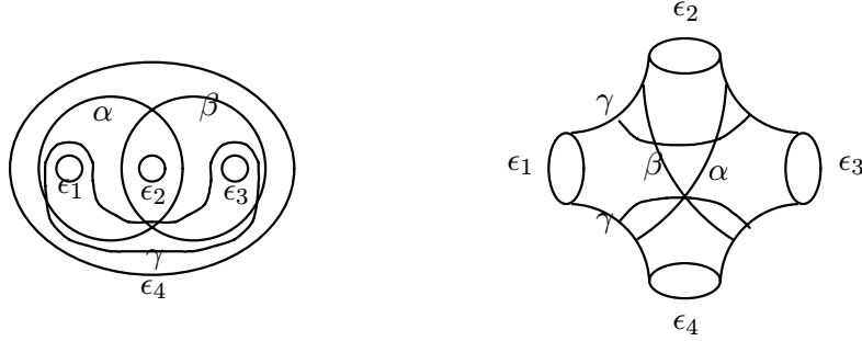
Figure 2. Two views of the curves that appear in the lantern identity on a sphere.
