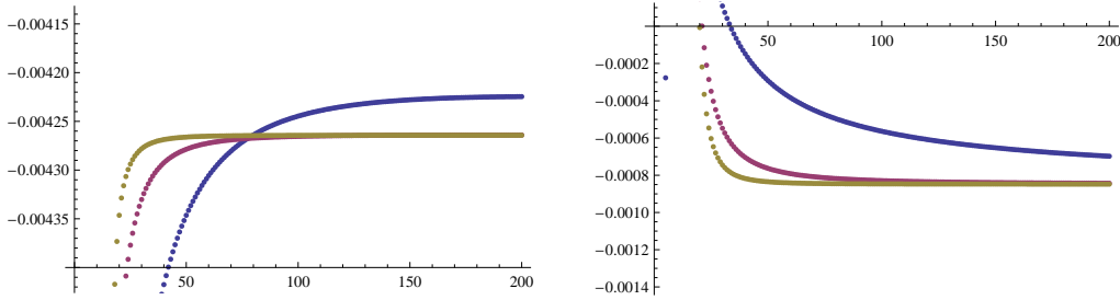
Figure 6. A plot of the sequence \tilde{b}_{m,k} , obtained from (5.30), together with its Richardson transformations, for k = 2 (left) and k = 5 (right).
