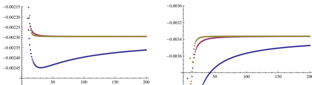
Figure 7. A plot of the sequence (5.39) and its Richardson transformations, for k = 2 (left) and k = 5 (right).
