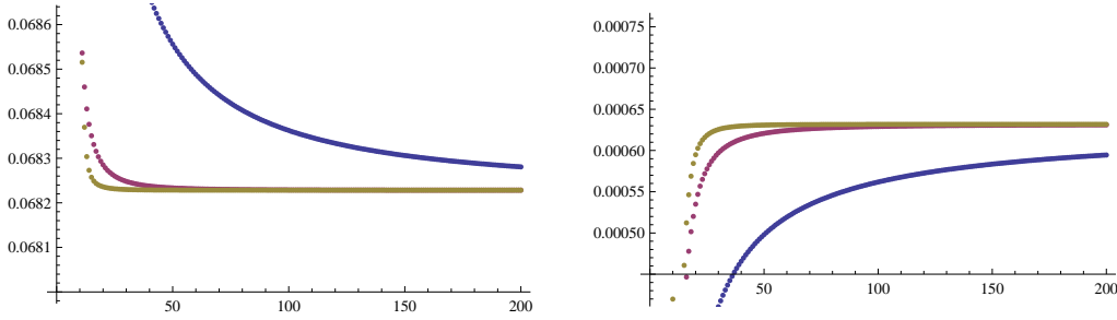
Figure 5. A plot of the sequence (5.26) and its Richardson transformations, for k = 2 (left) and k = 5 (right).
