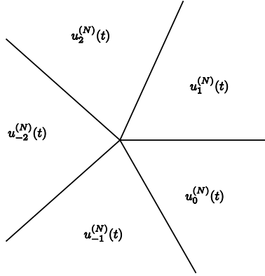
Figure 2. The sectorially meromorphic function \hat{u}^{(N)}(t) (2.16).
