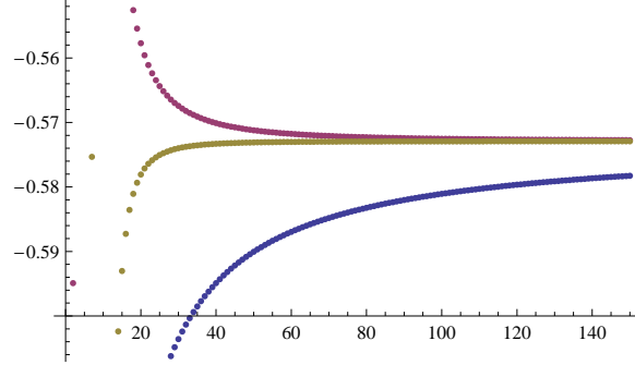
Figure 4. A plot of the sequence (5.17) and its Richardson transformations. In this and subsequent plots, the horizontal axis represents the integer n , and the vertical axis the values of the sequence.
