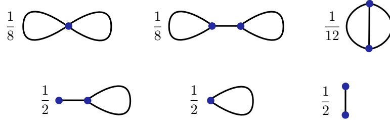
FIGURE 1. Diagrams contributing to S_{M,2} with symmetry factors. The top row of diagrams have exactly two loops, while the bottom row have fewer loops and additional 1-vertices and 2-vertices.
