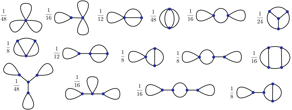
FIGURE 2. Diagrams with three loops contributing to S_3 .
