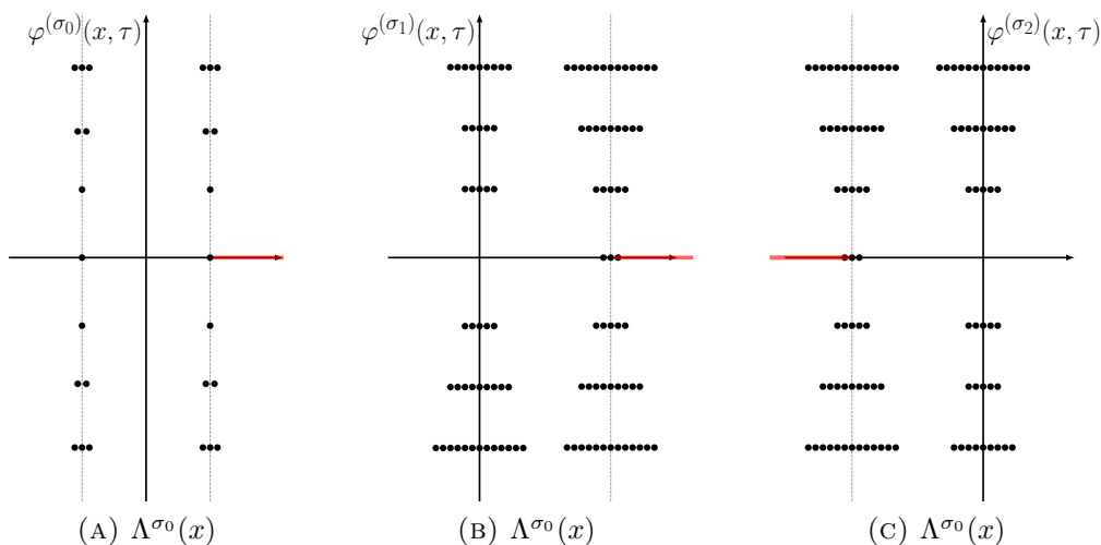
FIGURE 4. Singularities of the Borel transforms of \varphi^{(\sigma_j)}(x, \tau) for j = 0, 1, 2 of the knot 4_1 .
