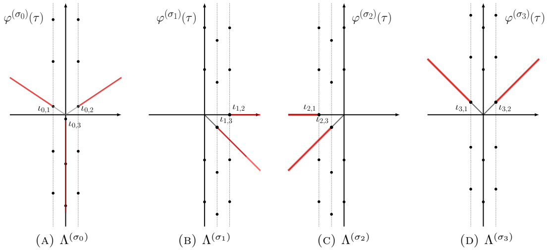
FIGURE 6. Singularities of Borel transforms of \varphi^{(\sigma_j)}(\tau) for j = 0, 1, 2, 3 of the knot \mathbf{5}_2 .
