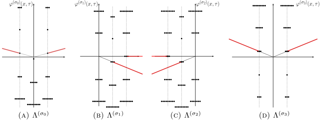
FIGURE 8. Singularities of Borel transforms of \varphi^{(\sigma_j)}(x, \tau) for j = 0, 1, 2, 3 of the knot \mathfrak{5}_2 .
