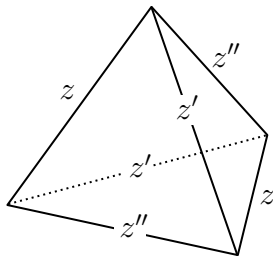
FIGURE 1. An ideal tetrahedron.
