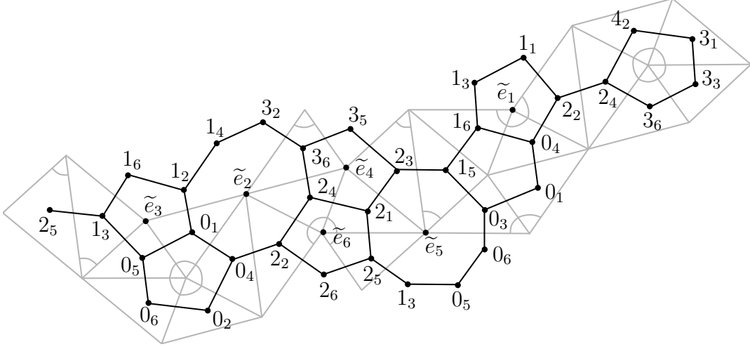
FIGURE 7. The dual 1-skeleton of \mathbb{E}^2 .
