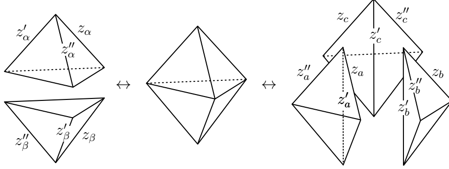
FIGURE 2. 2-3 Pachner move.
