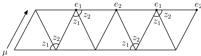
FIGURE 3. The triangulation of the peripheral torus of 4_1 .
