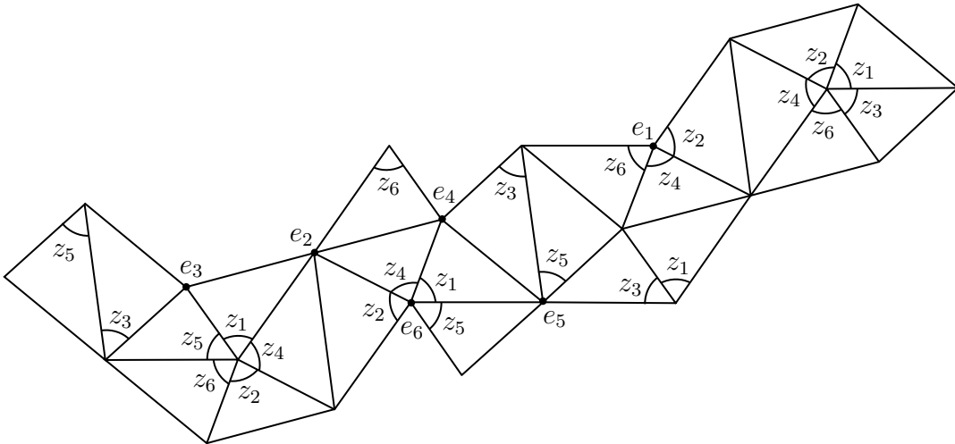
FIGURE 6. The triangulation of the peripheral torus of 6_3 .
